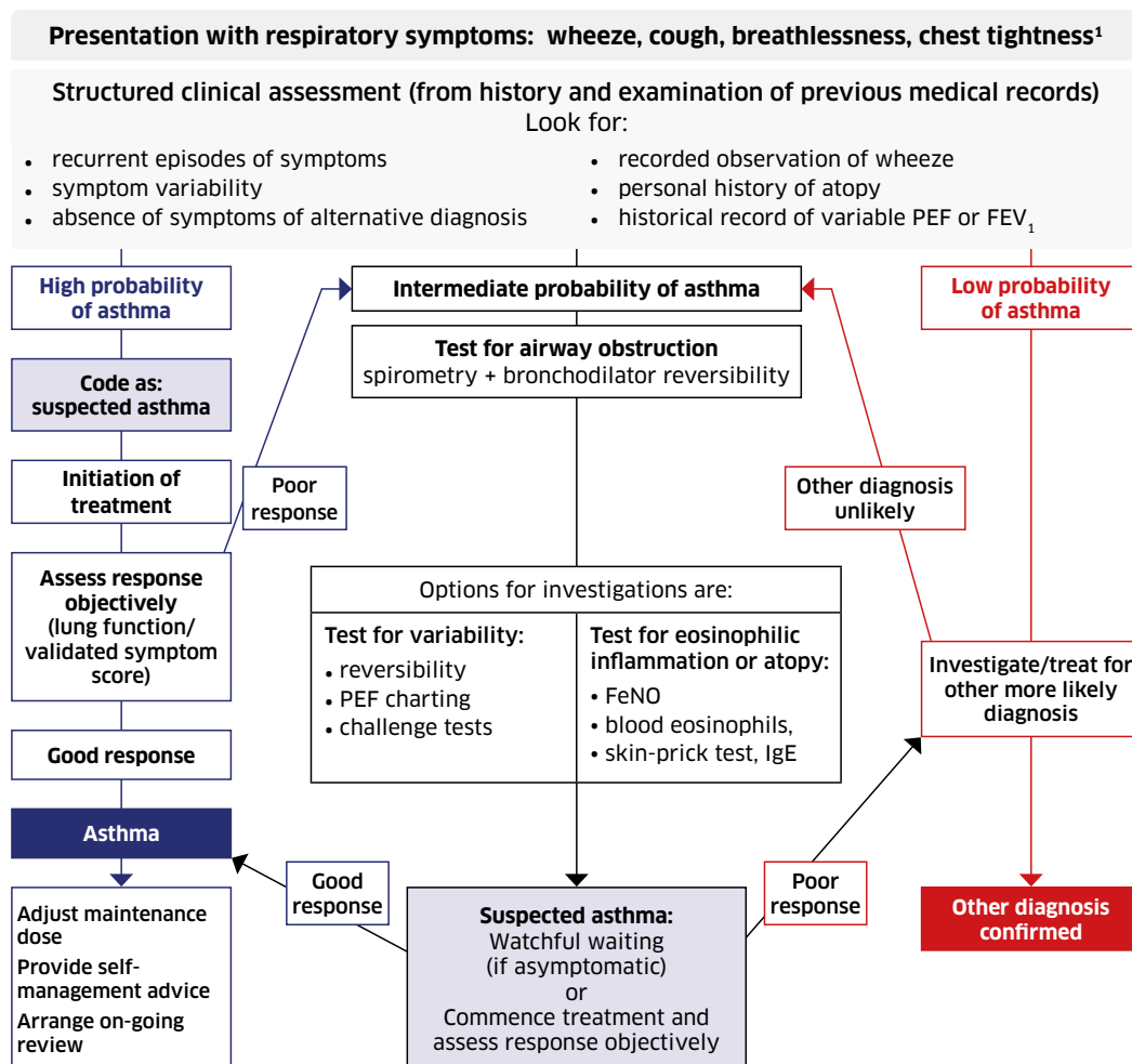
Figure 1: Diagnostic algorithm
